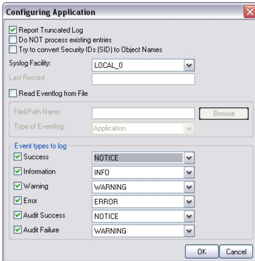
Event Log Monitor - EventLog Types Options
