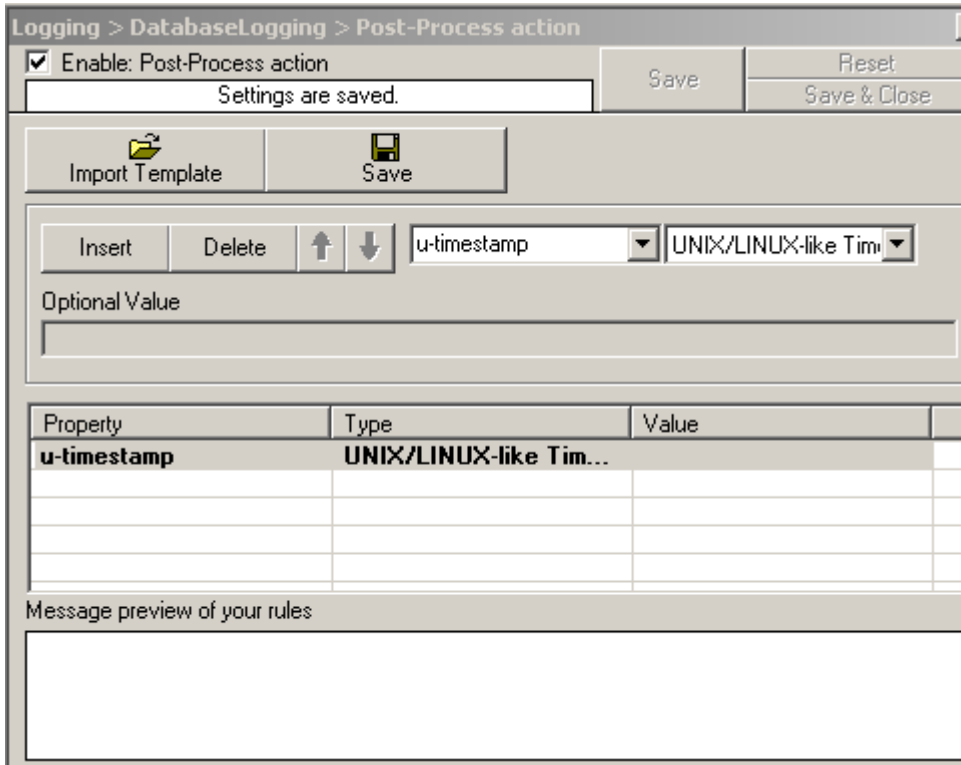
Post-Process Editor: Inserted a 'UNIX/LINUX like timestamp' rule
