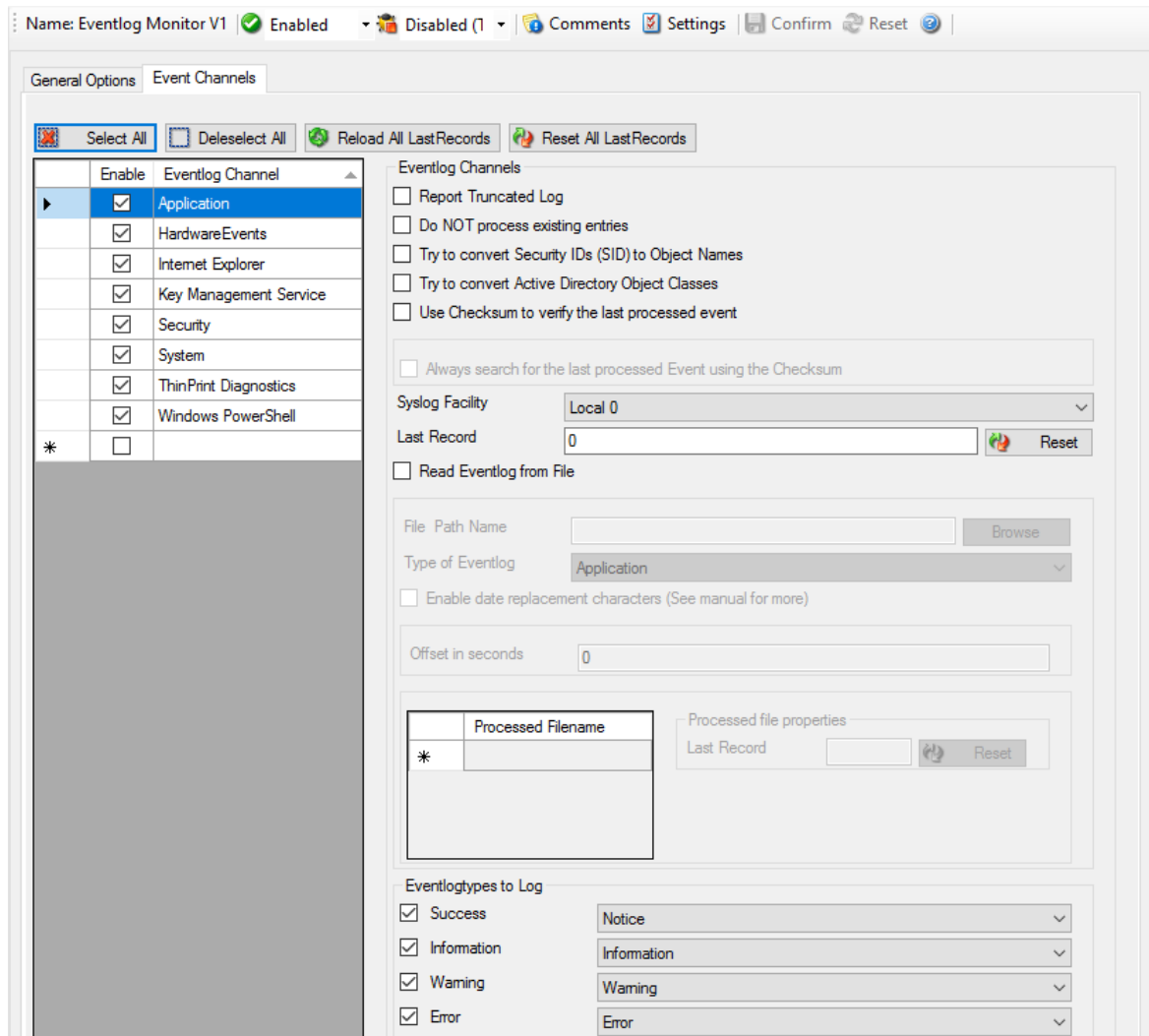
Event Log Monitor - EventLog Types General Options
