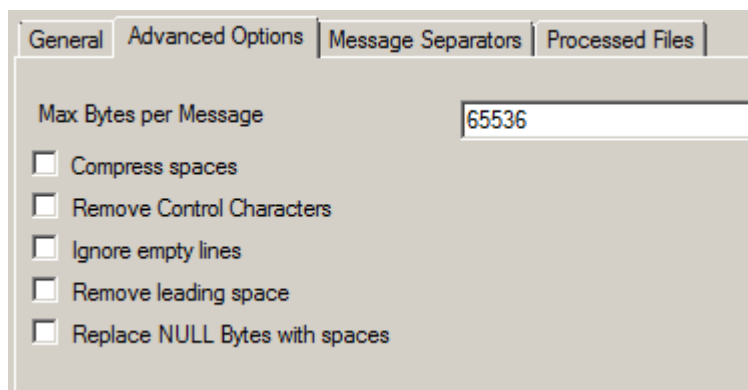
Figure 2: Advanced Options
