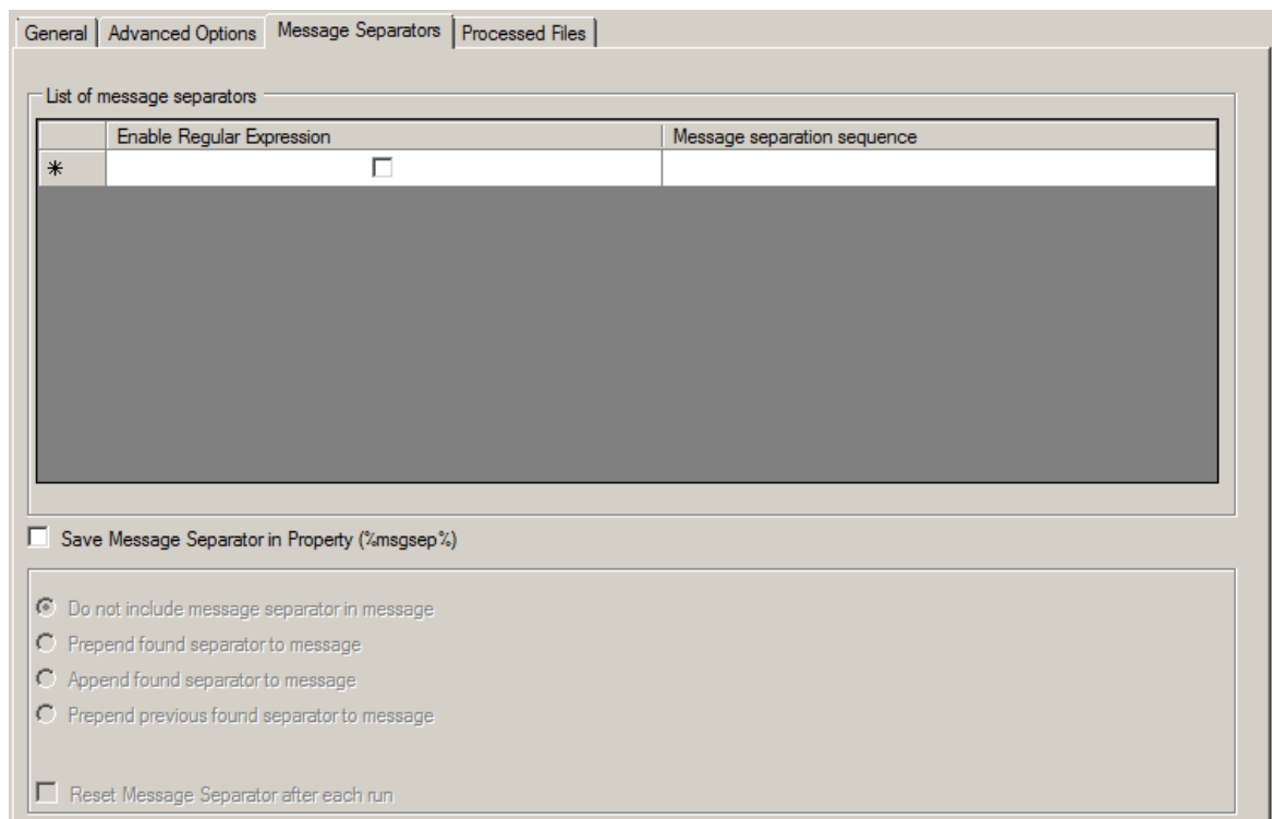
Figure 3: Message Separators
