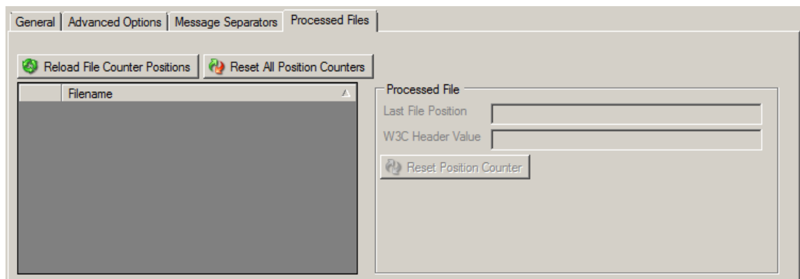
Figure 4: Processed Files
