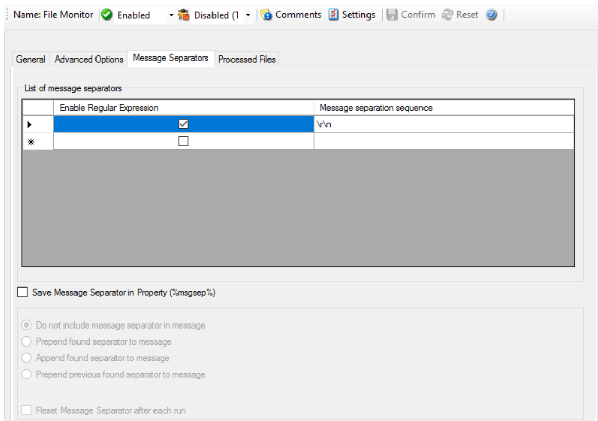
Figure 3: Message Separators
