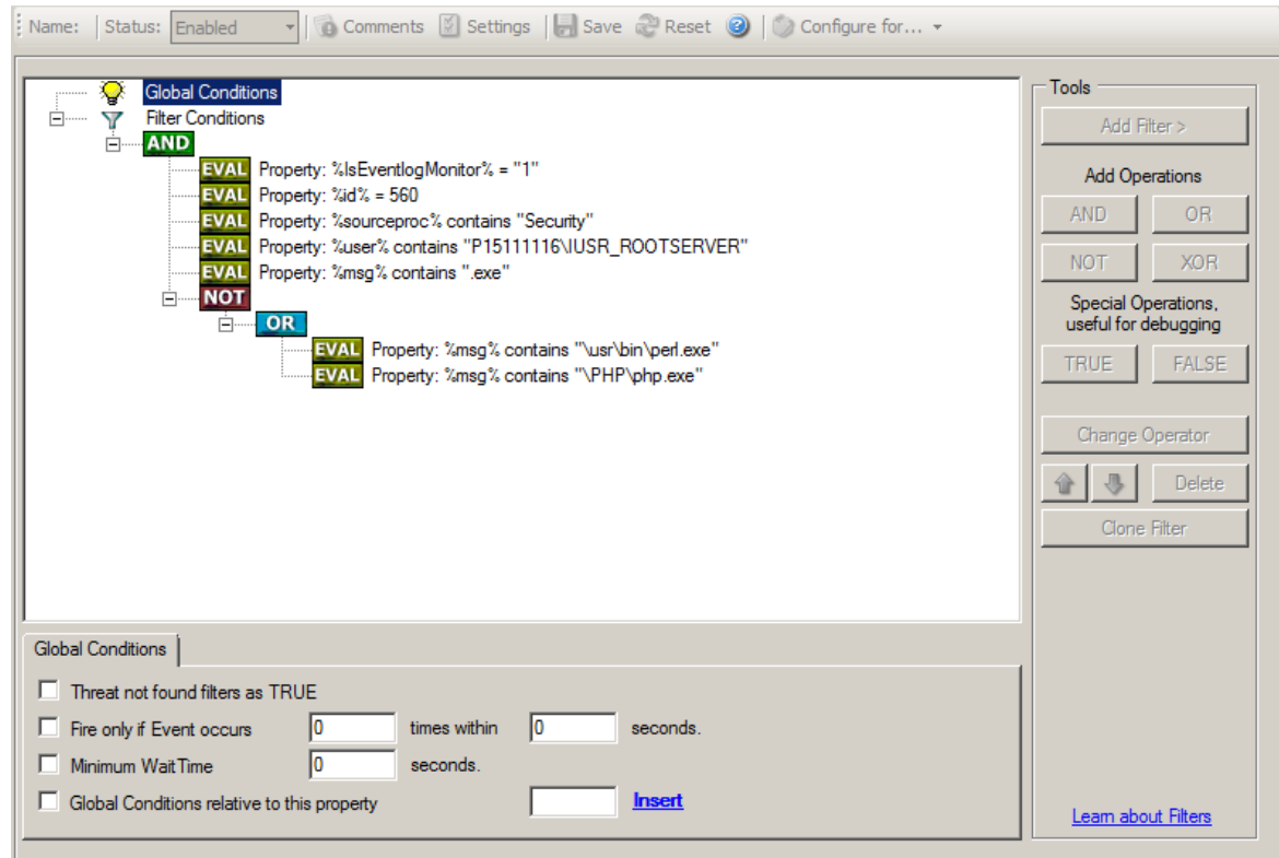
Filter Conditions - Complex Filter
