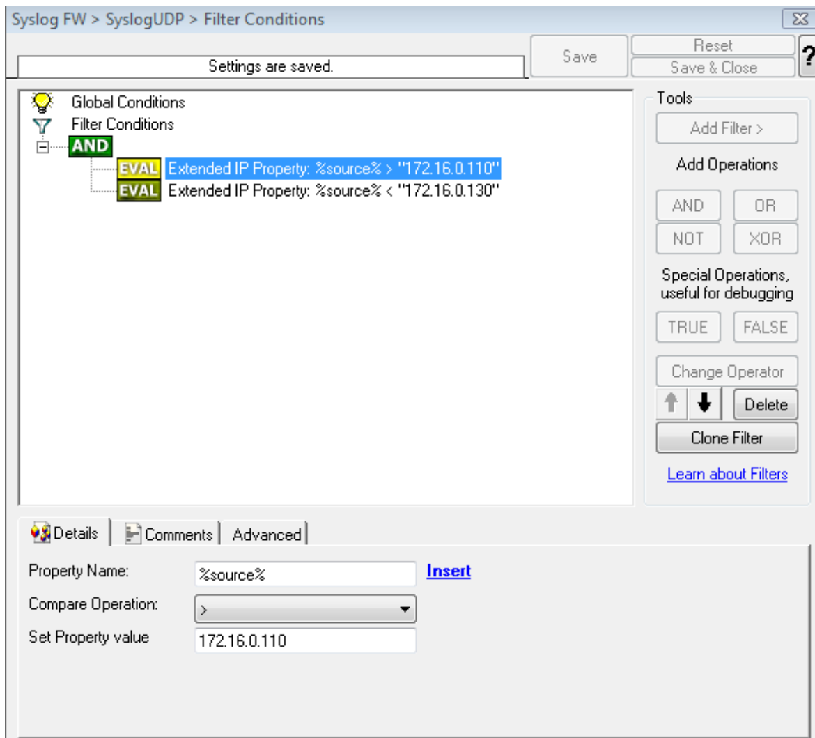
Filter Condition - Filtering for an IP Range
