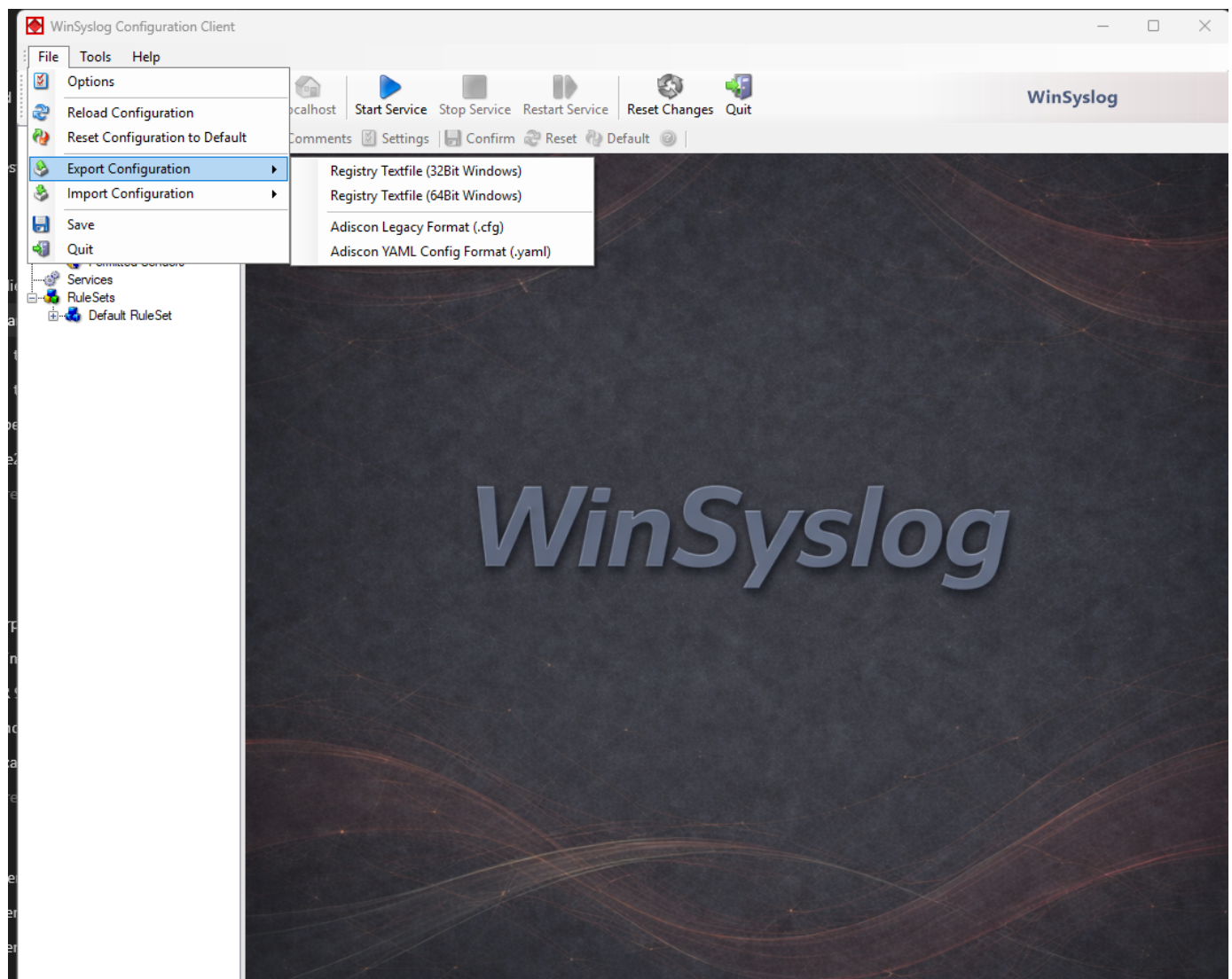
WinSyslog File menu with YAML import and export commands
