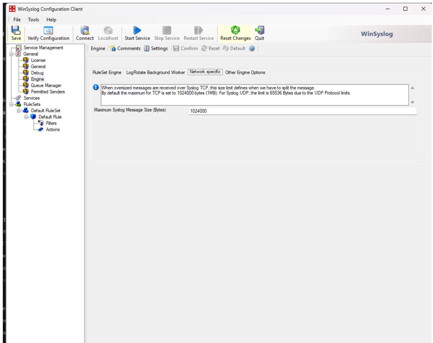
WinSyslog Network specific Options tab
