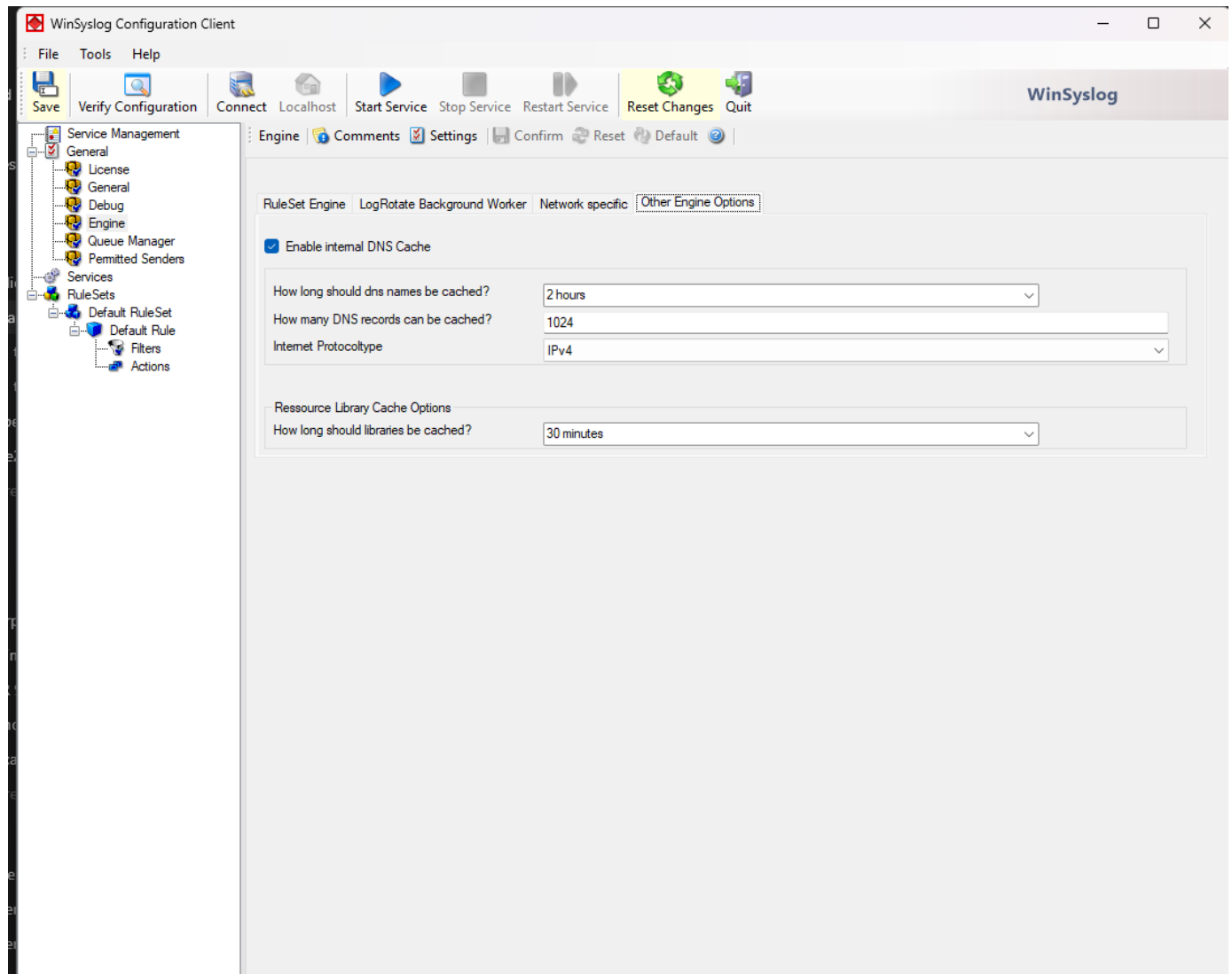
WinSyslog Other Engine Options tab
