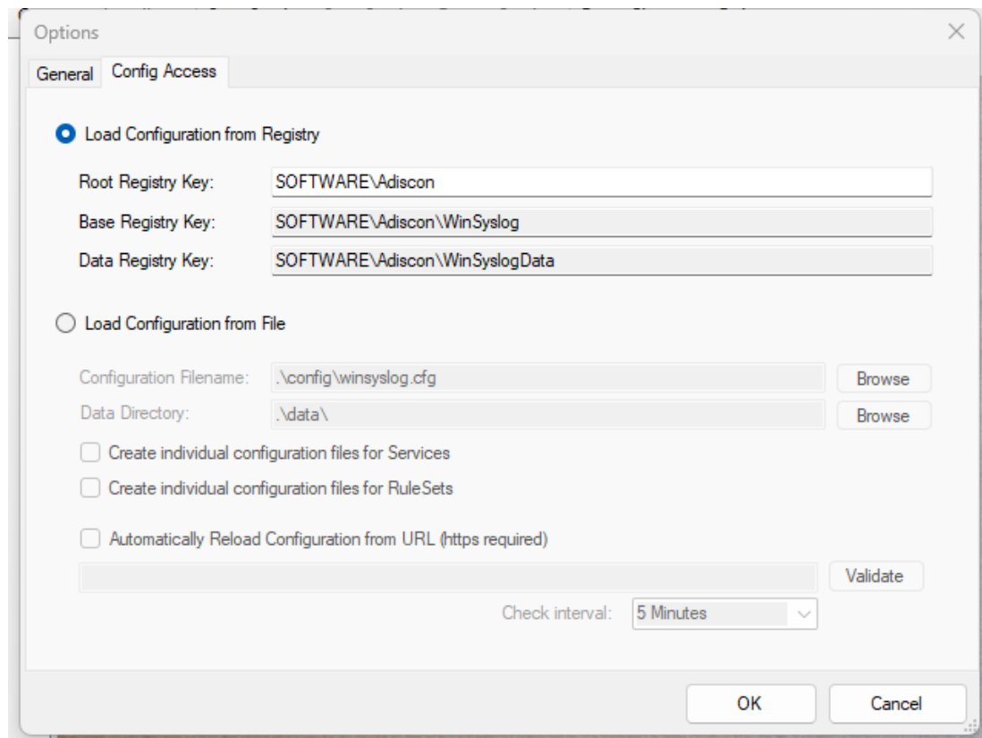
WinSyslog file-based configuration options
