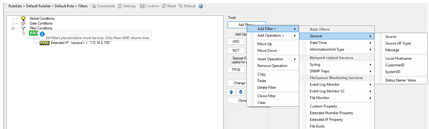
WinSyslog Filter Conditions - General
