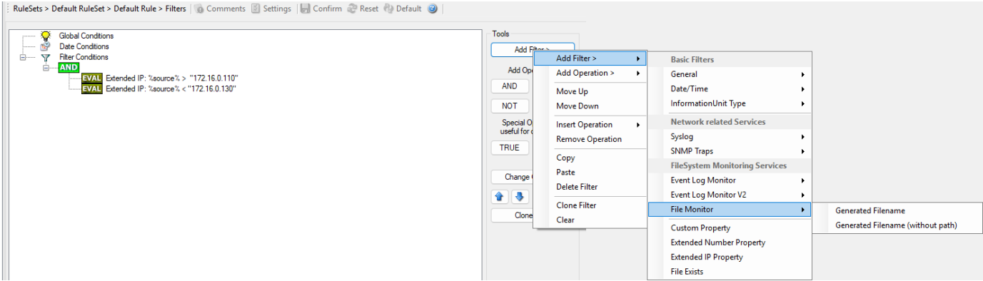
WinSyslog Filter Conditions - File Monitor
