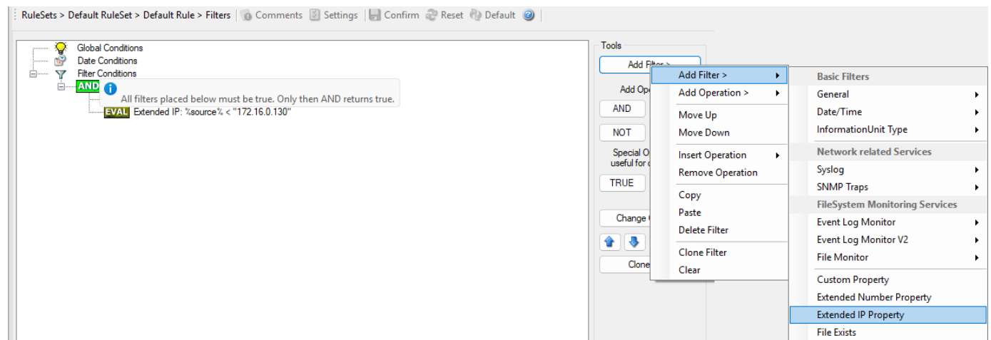
WinSyslog Filter Conditions - Extended IP Property
