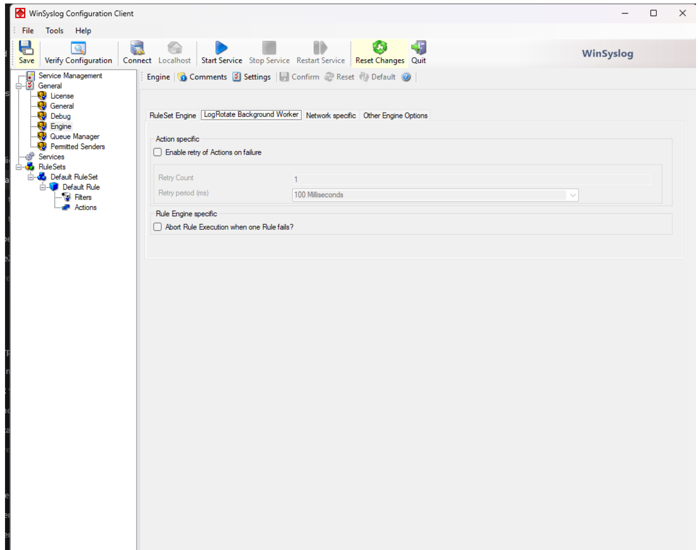
WinSyslog LogRotate Background Worker tab
